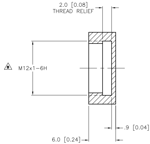
FULL SECTION
